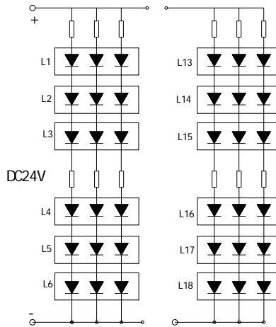
Circuit Diagram
