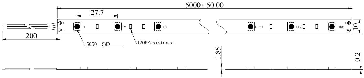
Dimension Drawing
