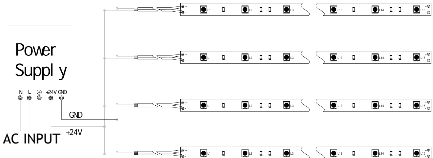
Installation drawing
